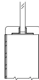
Veneered fire rated bead with metal clip system
