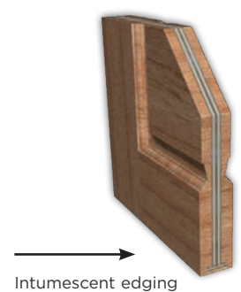
45-60-90 minute fire-rated door cross section
