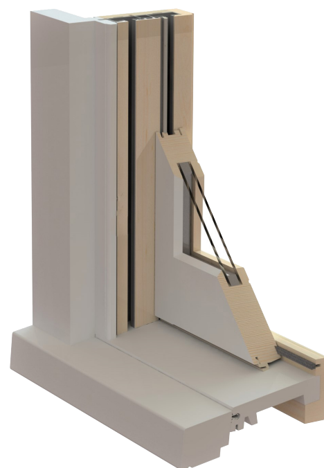
DHW350 (EW300) WITH 1 ¾" HISTORIC SILL NOSE 3 ½" FLAT EXTERIOR CASING
