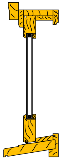
WOOD PICTURE DPW350 (EPW300)
