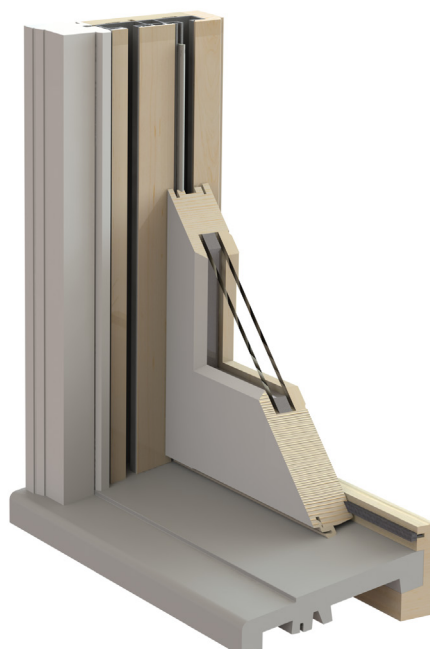
DHW350 (EW300) 1" STANDARD SILL 908 BRICKMOULD
