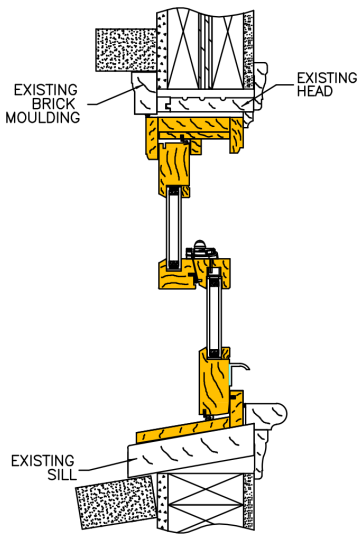
WOOD DOUBLE HUNG DHW250 (EW200)
