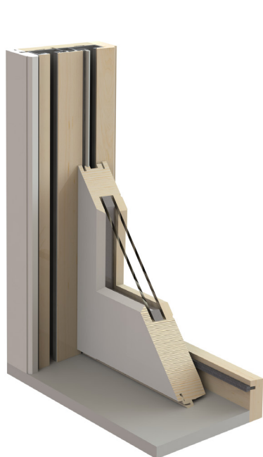
DHW250 (EW200) ½" REPLACEMENT SILL NO EXTERIOR CASING NO SCREEN STOP
