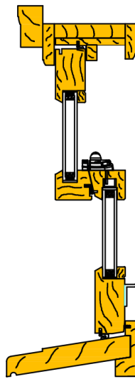
WOOD DOUBLE HUNG DHW350 (EW300)
